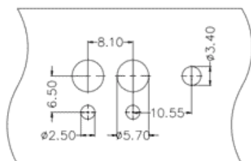
钻孔图 For a drilling diagram
